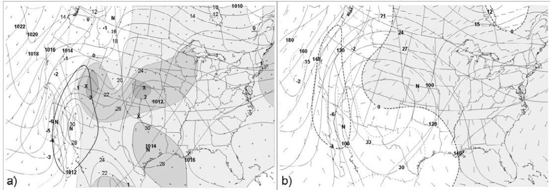
Figure 4. a) Composite of sea level pressure (hPa, bold), air temperature ( ^{\circ}\text{C} ), and surface thermal advection ( \times 10^{-1}^{\circ}\text{C hr}^{-1} , bold characters and dashed lines; shaded represents warm air advection) for the seven longest summer PPTAs. b) Composite of 1000hPa thermal advection ( \times 10^{-1}^{\circ}\text{C hr}^{-1} , dashed lines; shading represents warm air advection), heights (gpm, solid lines), air temperature ( ^{\circ}\text{C} ) and wind ( \text{m}\cdot\text{s}^{-1} ) for the seven longest summer PPTAs
