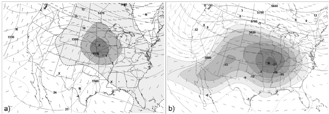
Figure 5. a) Composite of 850hPa thermal advection ( \times 10^{-1}^{\circ}\text{C day}^{-1} , dashed lines; shaded represents warm air advection), heights (gpm, solid lines), air temperature ( ^{\circ}\text{C} ) and wind ( \text{m}\cdot\text{s}^{-1} ) for the seven longest summer PPTAs. b) Composite of 500hPa vorticity advection ( \times 10^{-5}\cdot\text{s}^{-1} , dashed lines; shaded is negative vorticity), heights (gpm, solid lines), and winds ( \text{m}\cdot\text{s}^{-1} ) for the seven longest summer PPTAs
