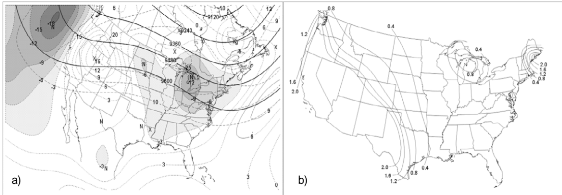
Figure 6. a) Composite of 300hPa divergence ( \times 10^{-6} \text{day}^{-1} , dashed lines; shaded represents convergence), height (gpm, solid lines), and isotachs ( \text{m}\cdot\text{s}^{-1} ) for the seven longest summer PPTAs. b) Composite of Bowen ratio for the seven longest summer PPTAs
